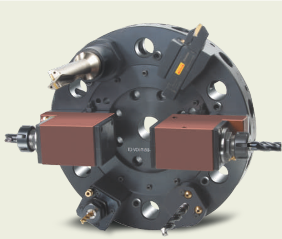
VDI TOOL DISC & TOOL HOLDERS
